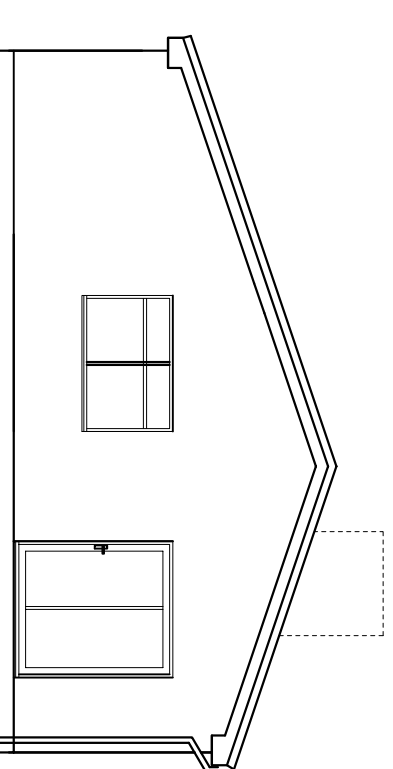
PROPOSED REAR
