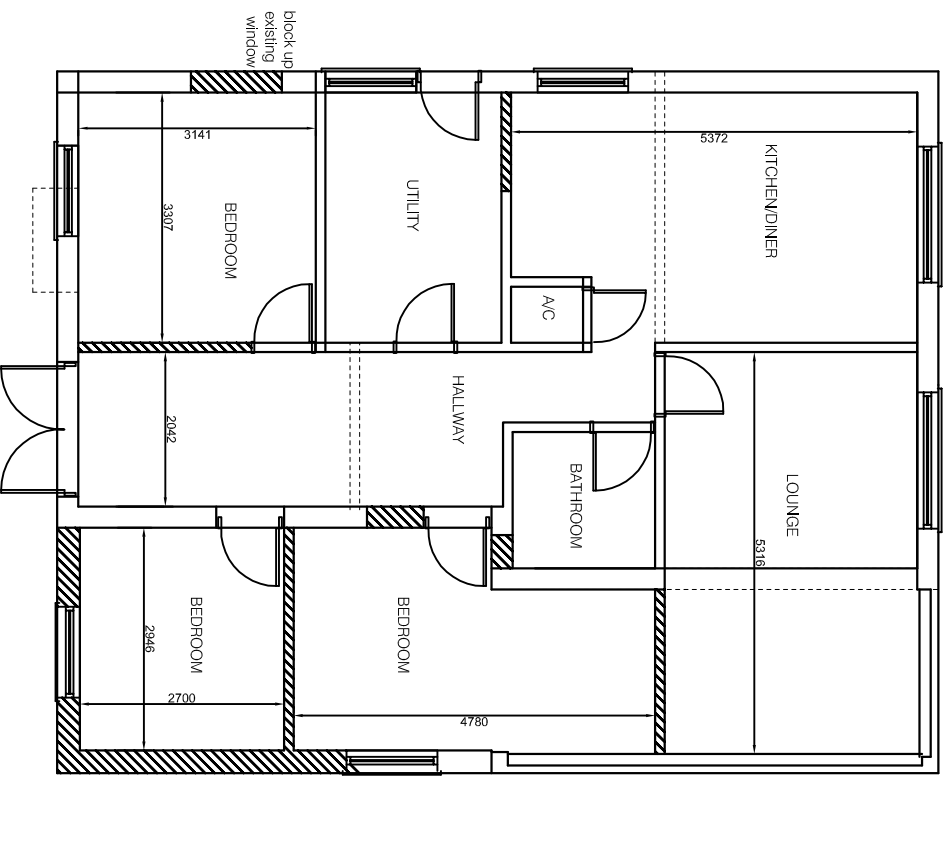
PROPOSED GROUND
