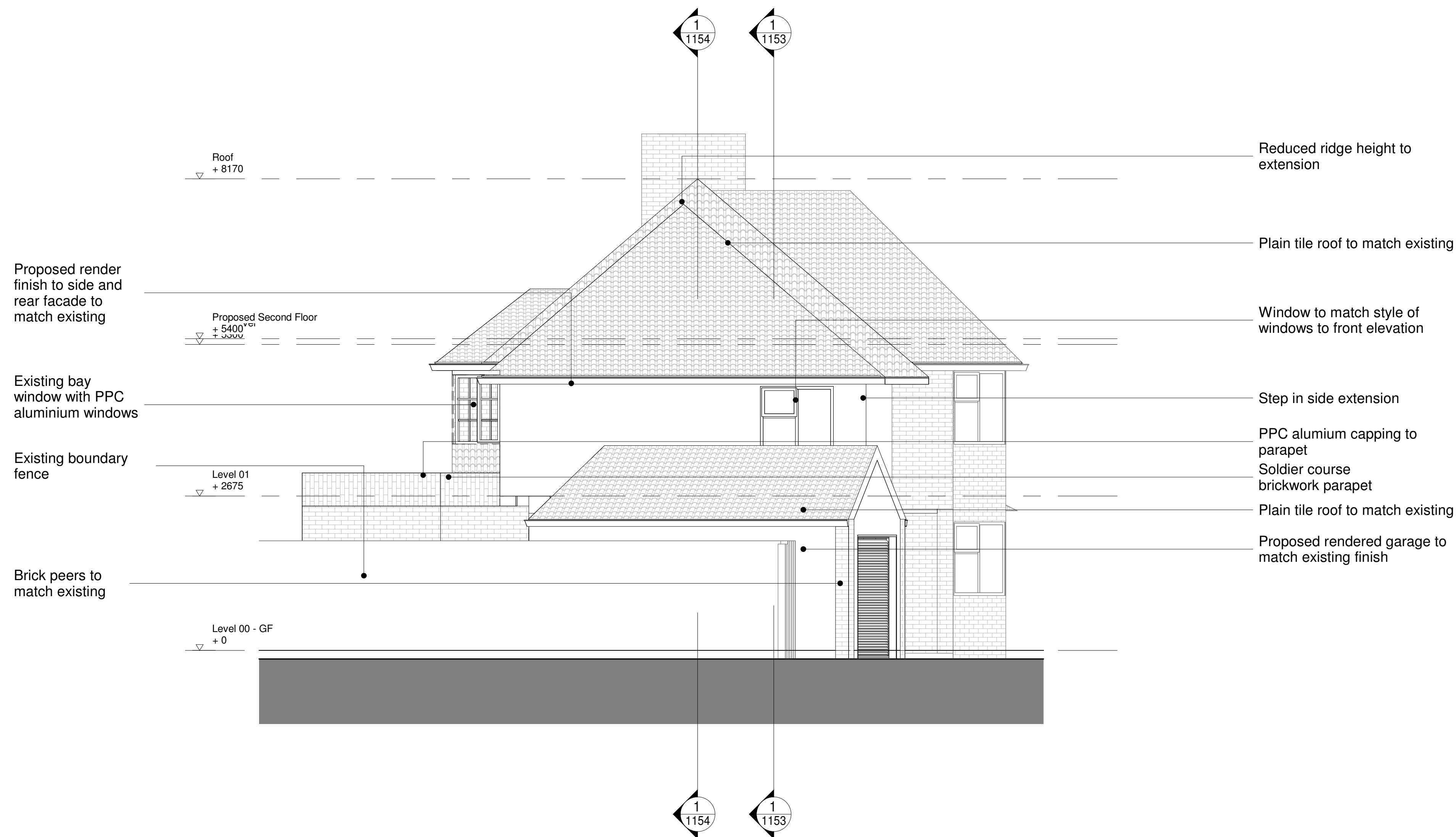
1 Proposed Elevation_Side 1 : 50
