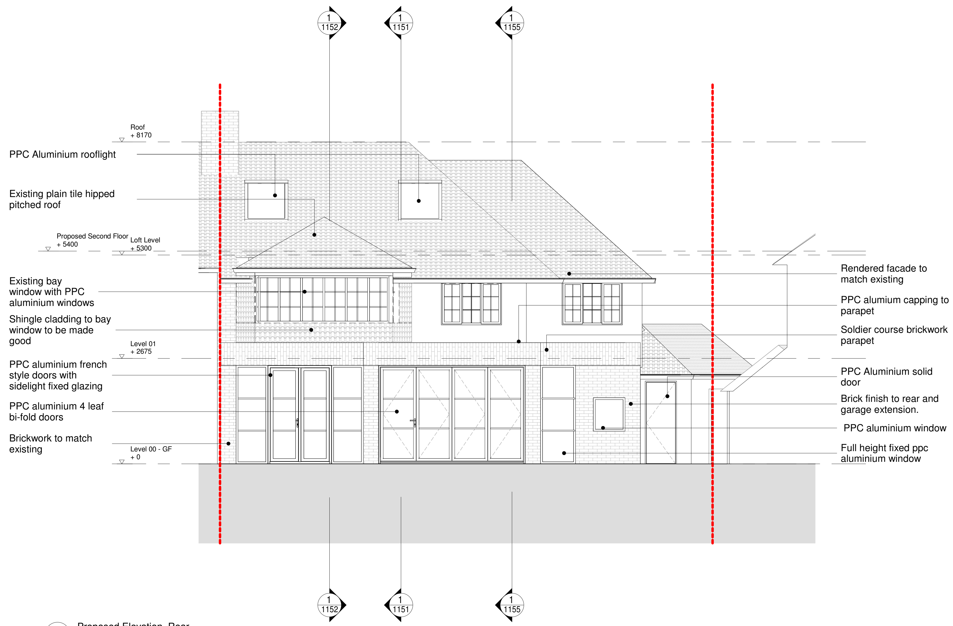
1 Proposed Elevation_Rear 1 : 50
