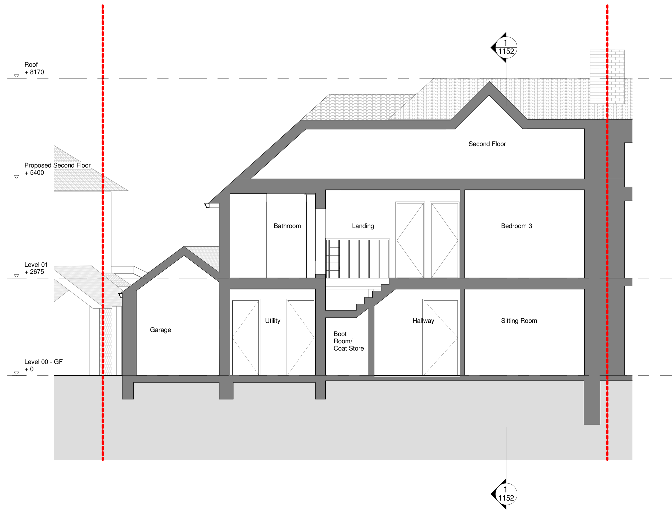
1 Proposed GA Section_C-C 1 : 50
