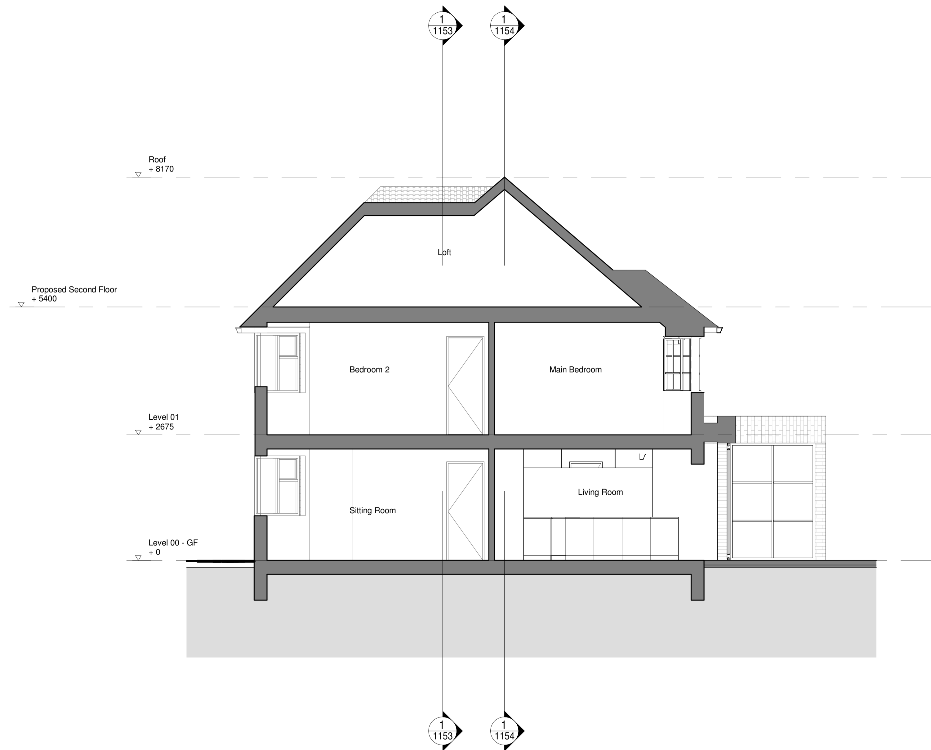
1 Proposed GA Section_B-B 1 : 50
