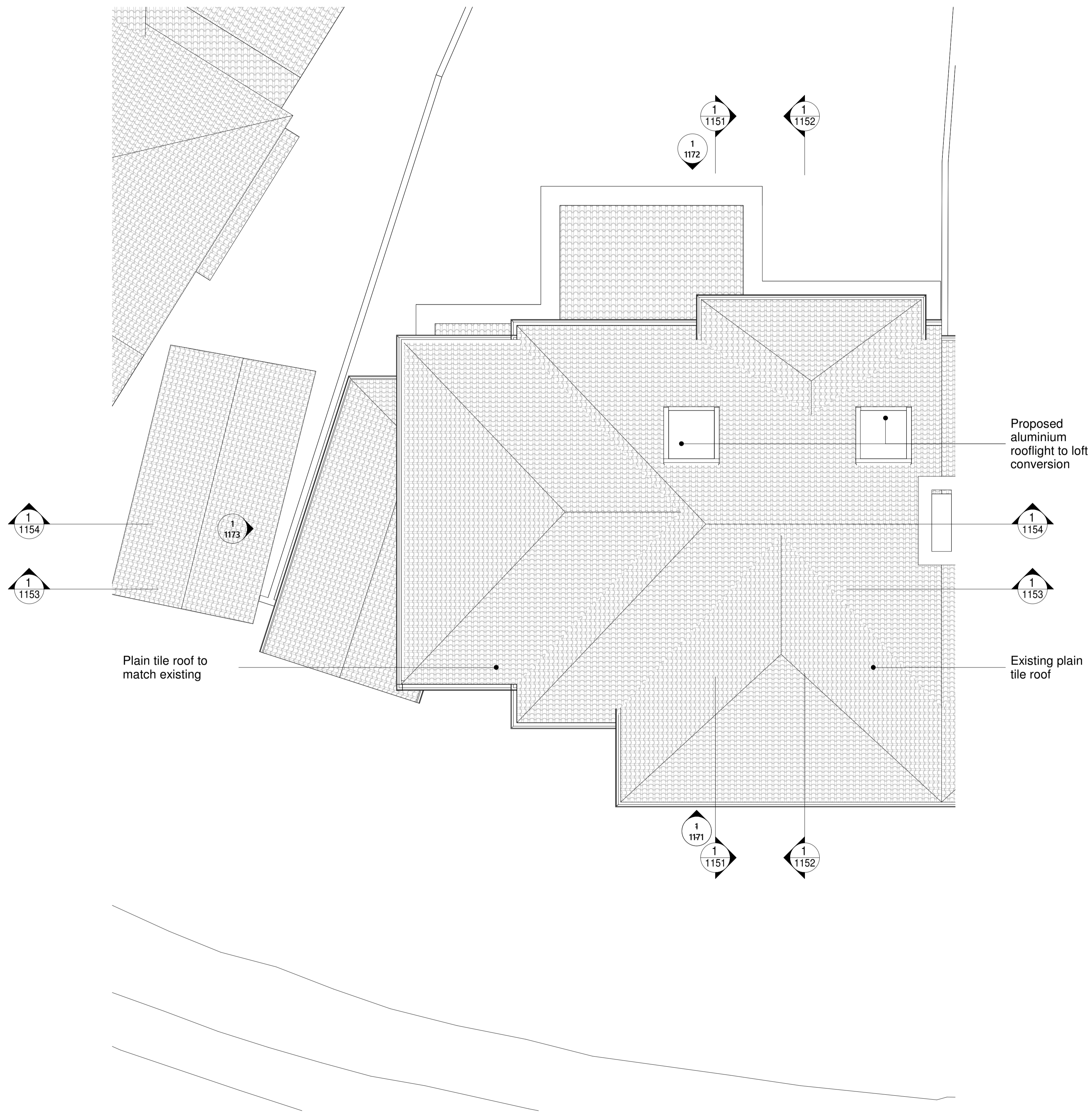
1 Proposed GA_Roof Plan_Level RF 1 : 50
