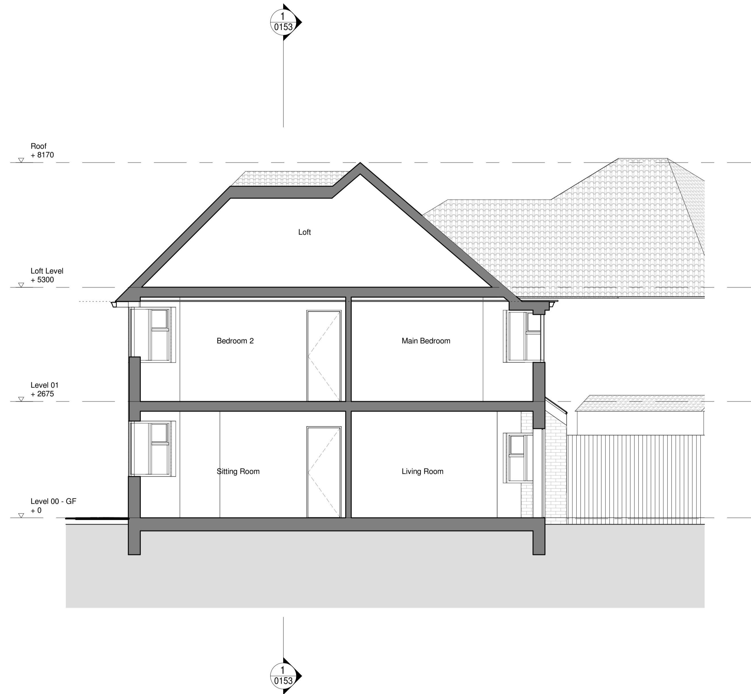
1 Existing Section_B-B 1 : 50
