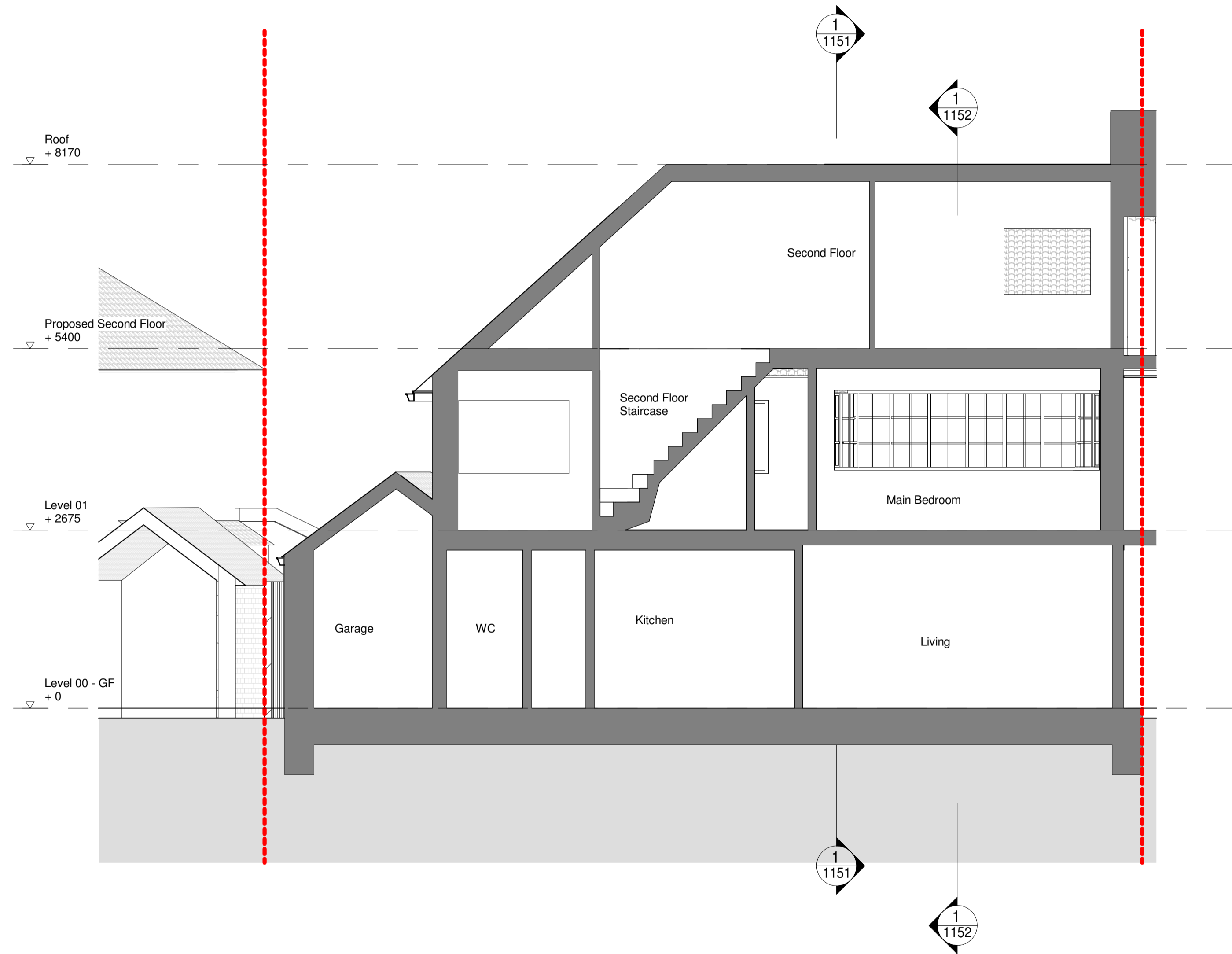
1 Proposed GA Section_C-C 1 : 50
