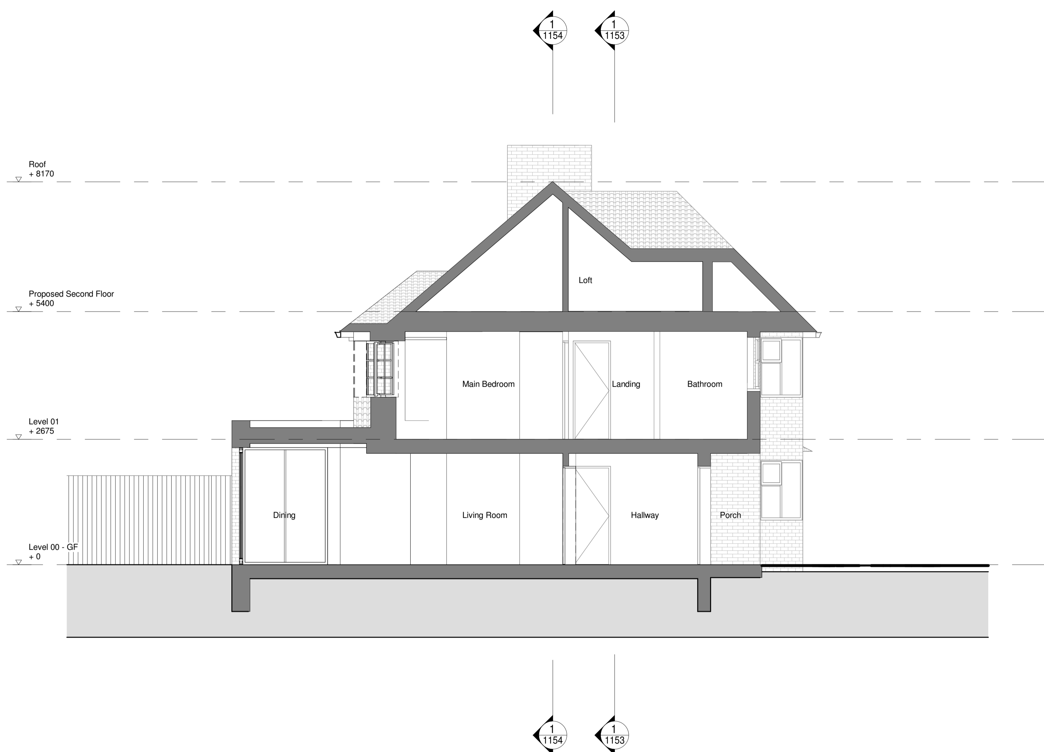
1 Proposed GA Section_A-A 1 : 50
