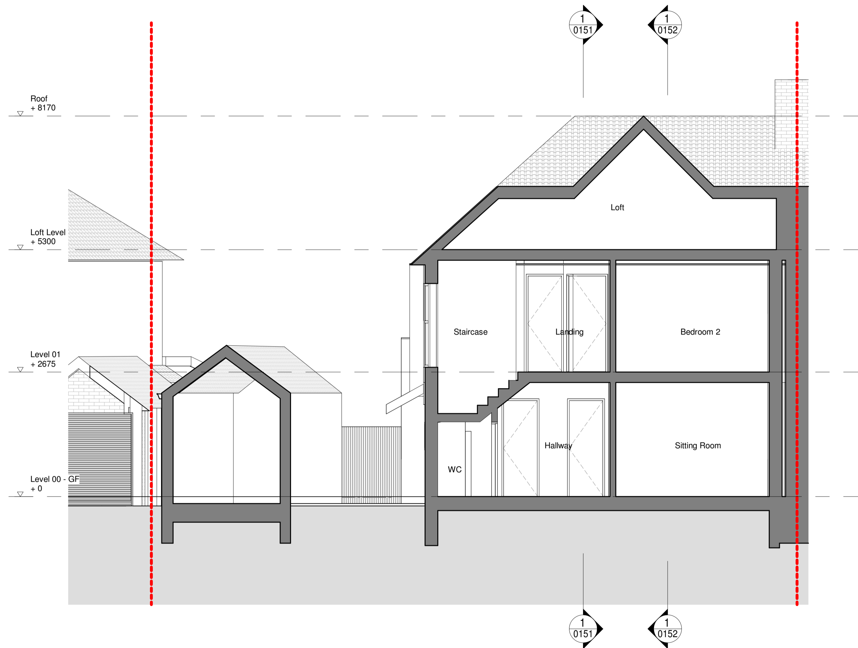
1 Existing Section_C-C 1 : 50
