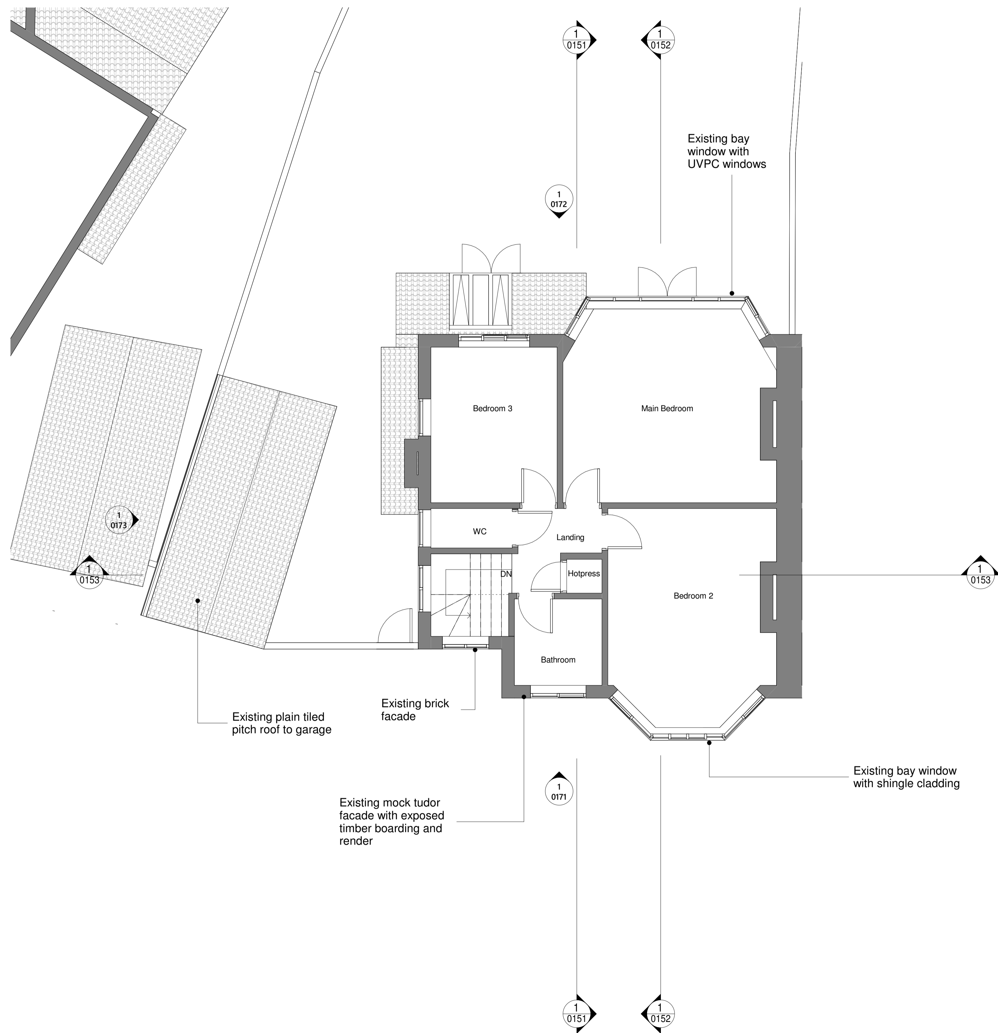
1 Existing Plan_First Floor_Level 01 1 : 50
