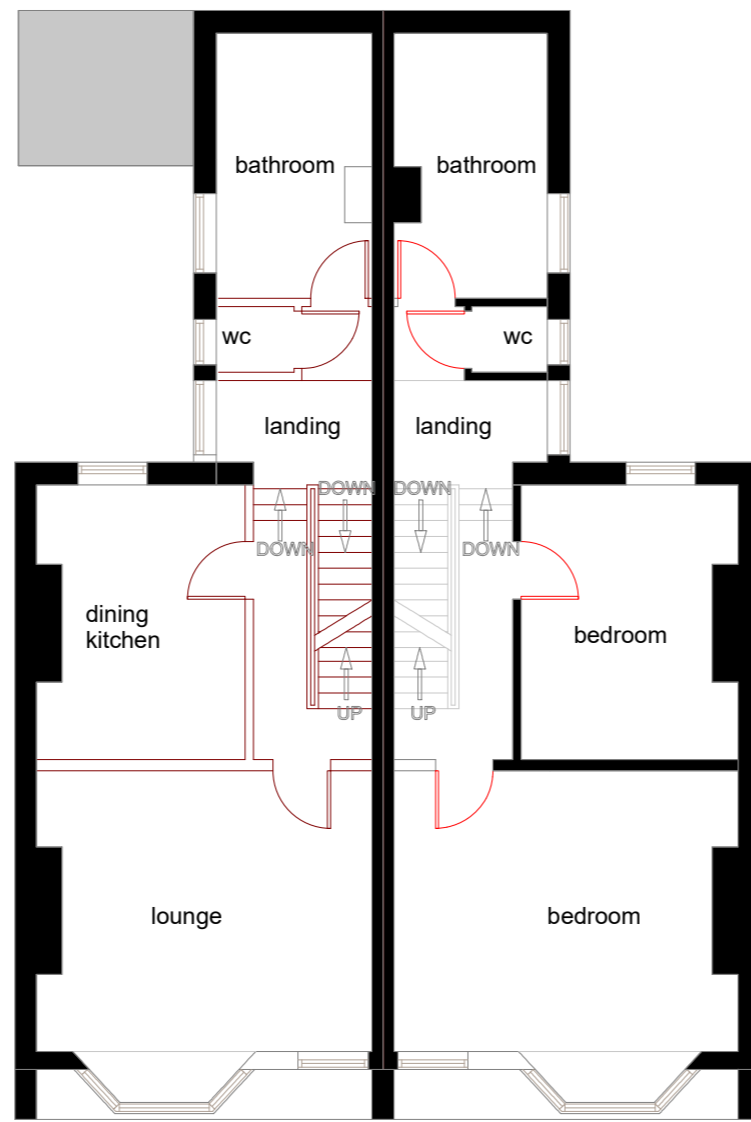
flat 2 first floor - existing
