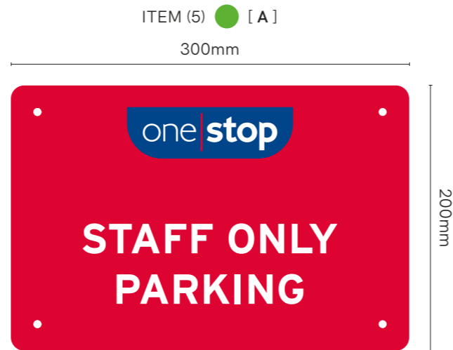
CAR PARK SIGN (wall mounted) scale 1:4 @ A3
