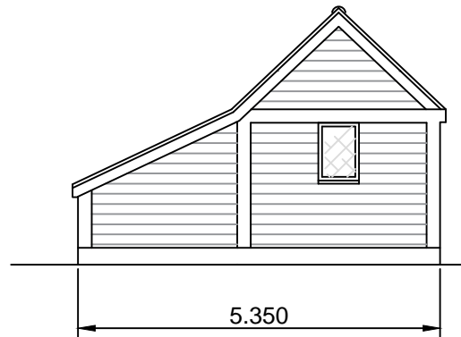
Left Elevation
