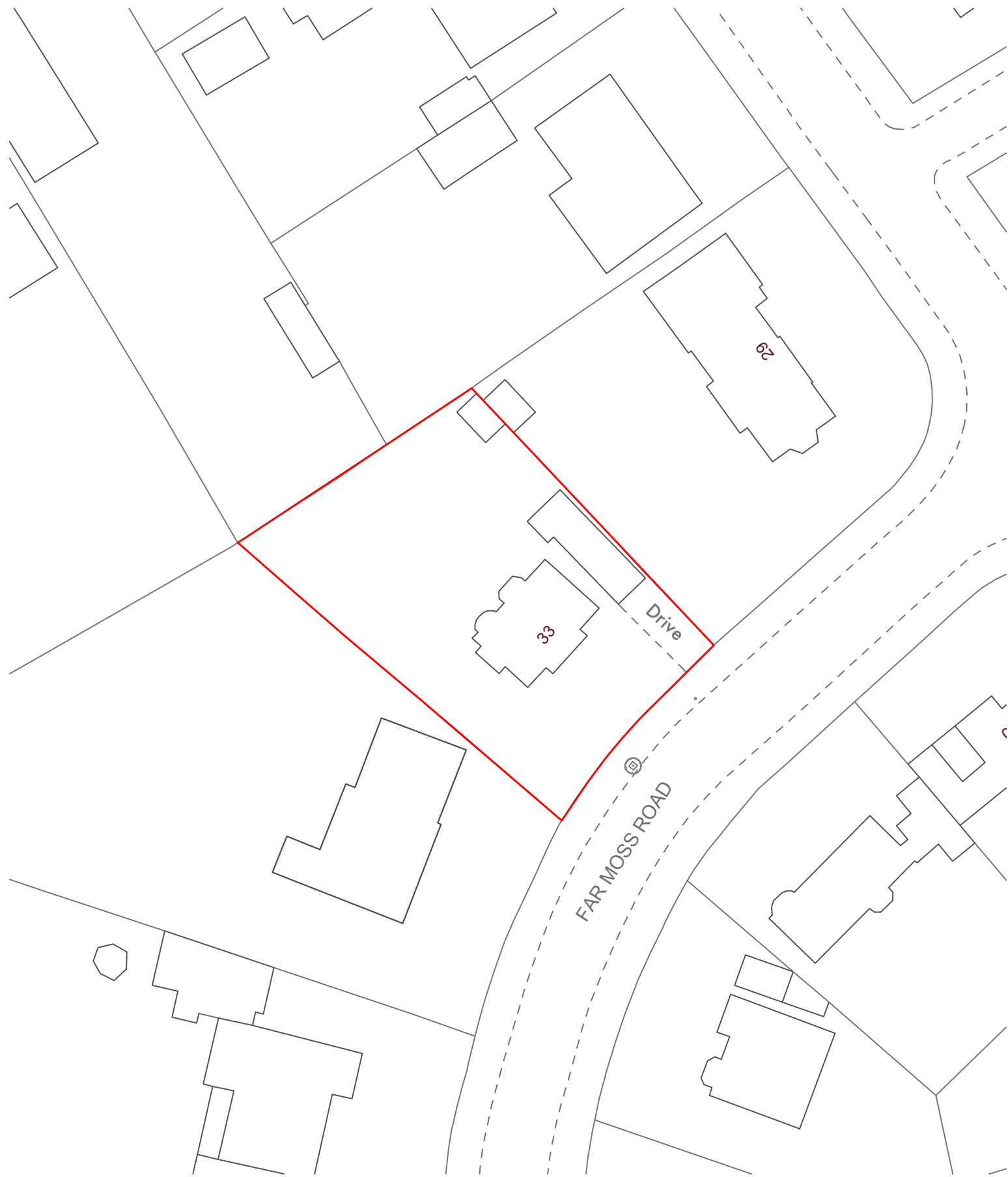
Site Plan @ 1:500
