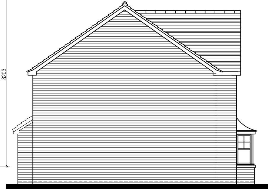
GABLE ELEVATION
