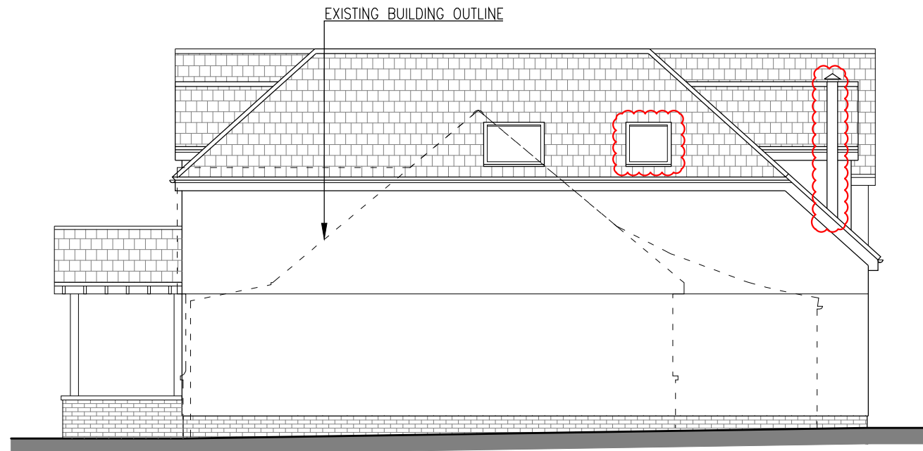
PROPOSED NORTH ELEVATION SC. 1:100 @ A3
