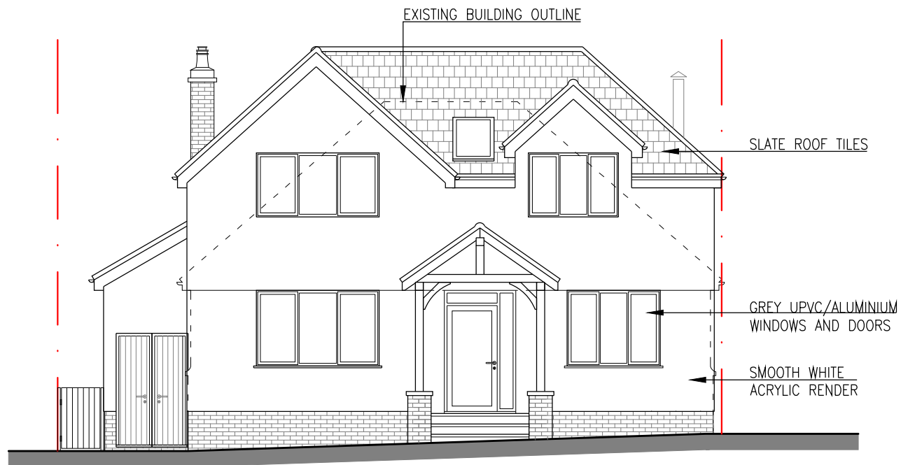
PROPOSED WEST ELEVATION SC. 1:100 @ A3
