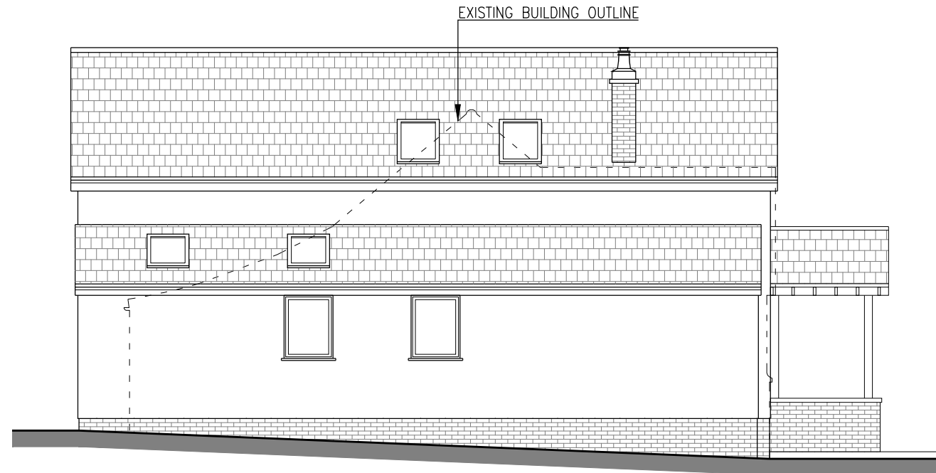
PROPOSED NORTH ELEVATION SC. 1:100 @ A3
