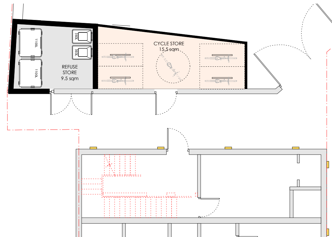
3 Proposed Refuse & Cycle Store 1:100 @ A3
