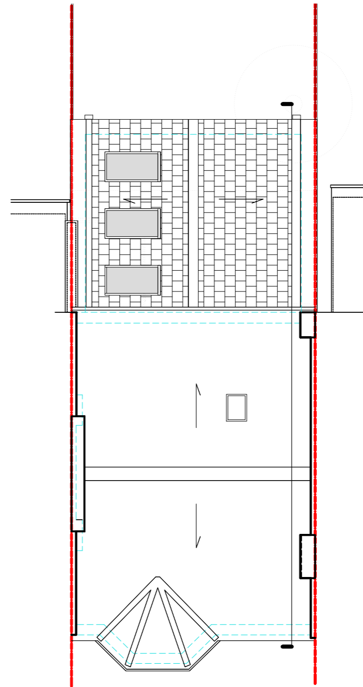
Roof plan 1:100
