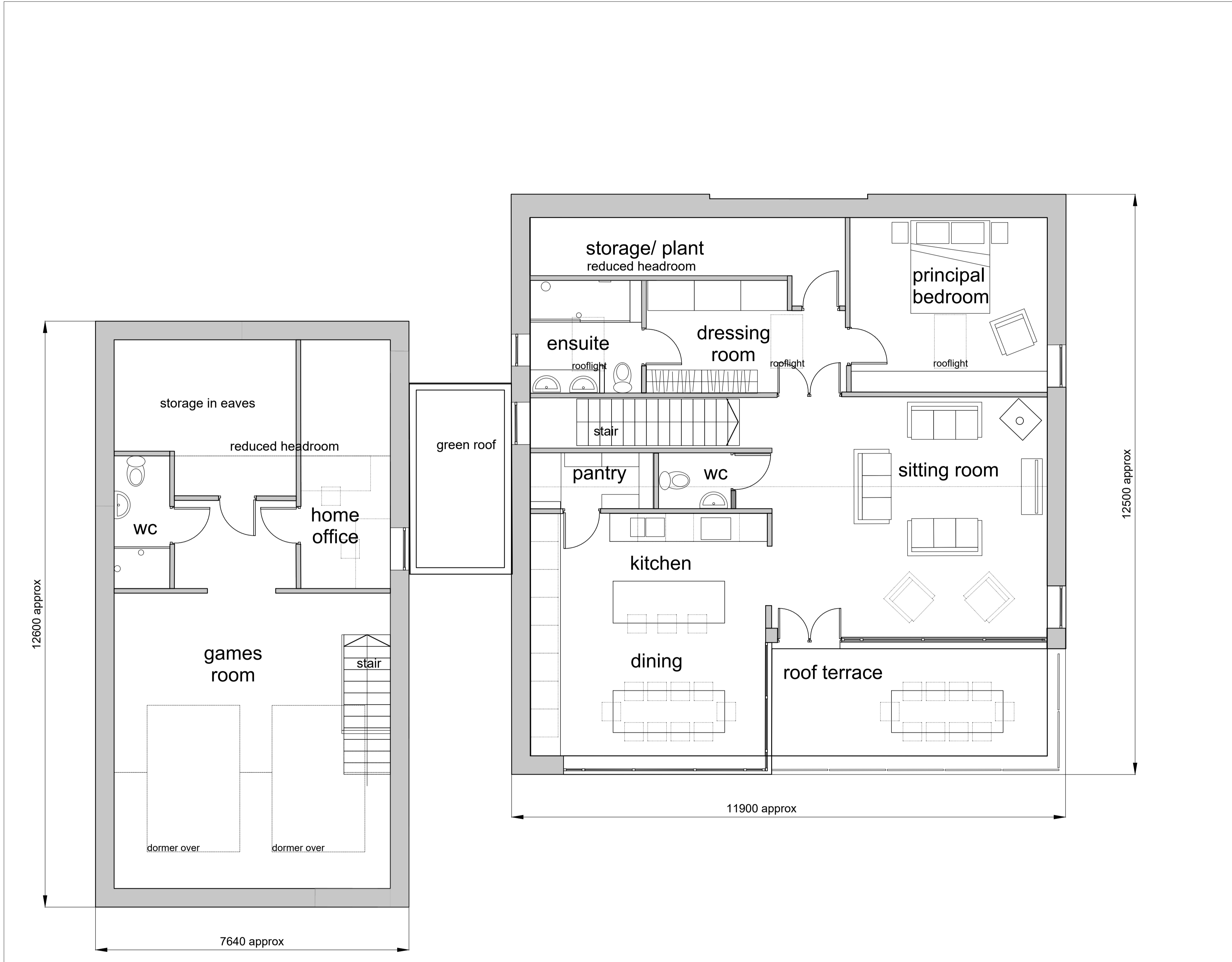
Plan, First Floor Level
