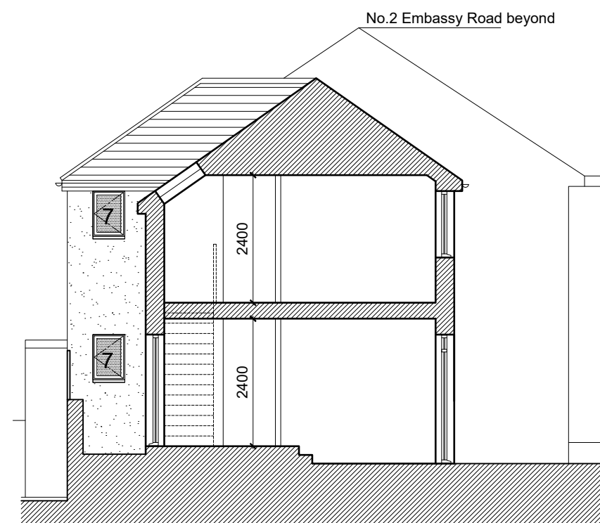
SECTION C-C
