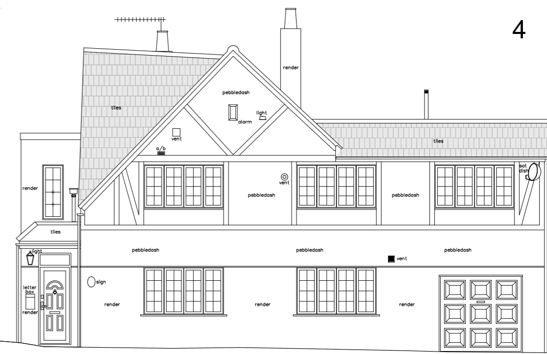
STREET SIDE ELEVATIONS 4,6 & 8 / EXISTING
