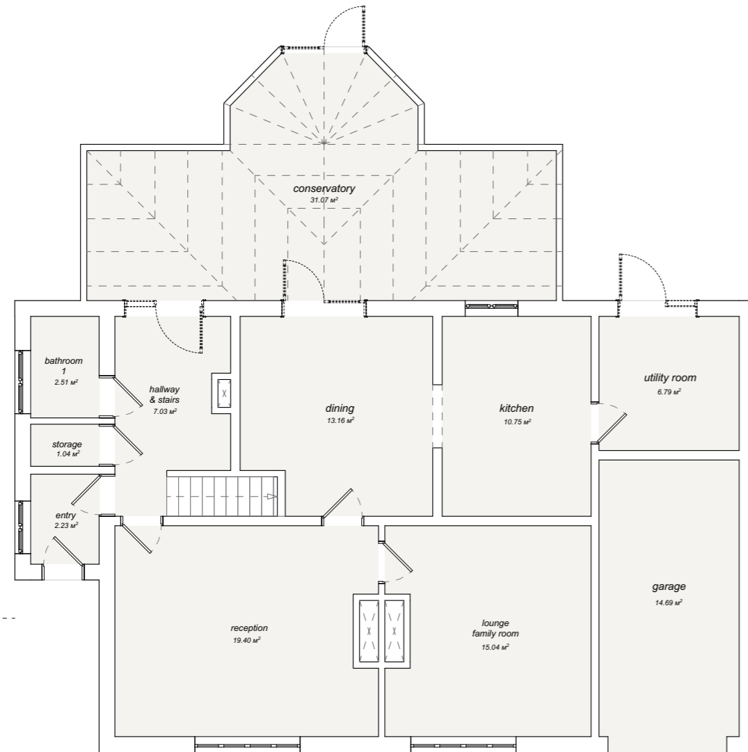
GROUND FLOOR PLAN EXISTING GIA: 124 sqm
