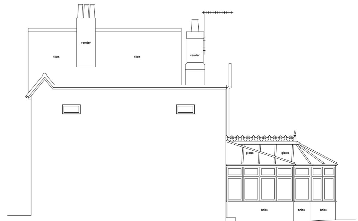
NORTH SIDE ELEVATION EXISTING
