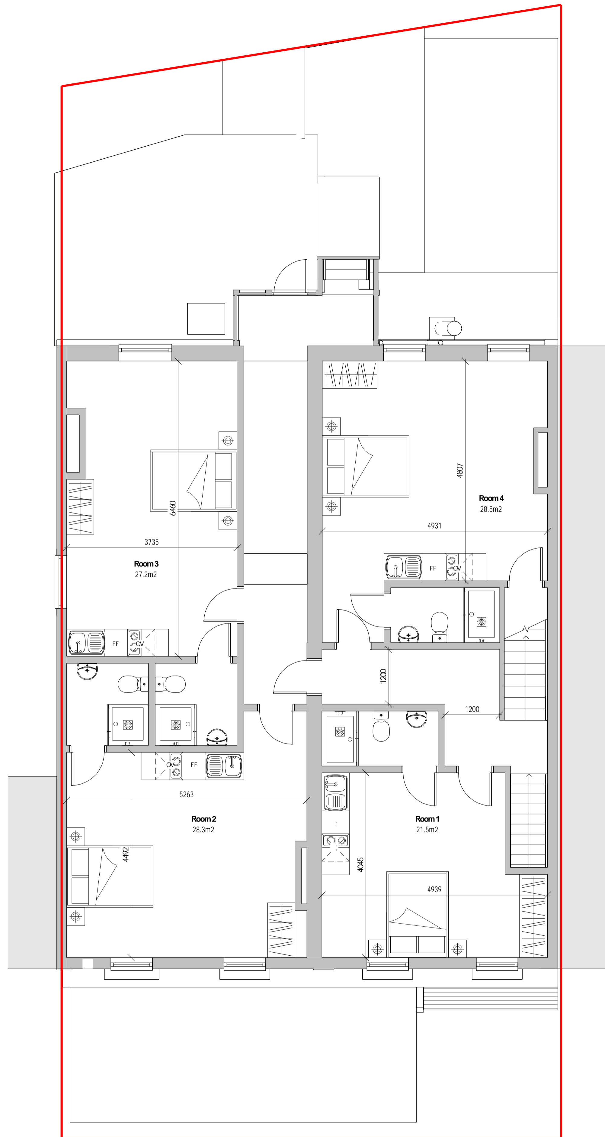
First Floor -GA Plan (Proposed) 1 : 50
