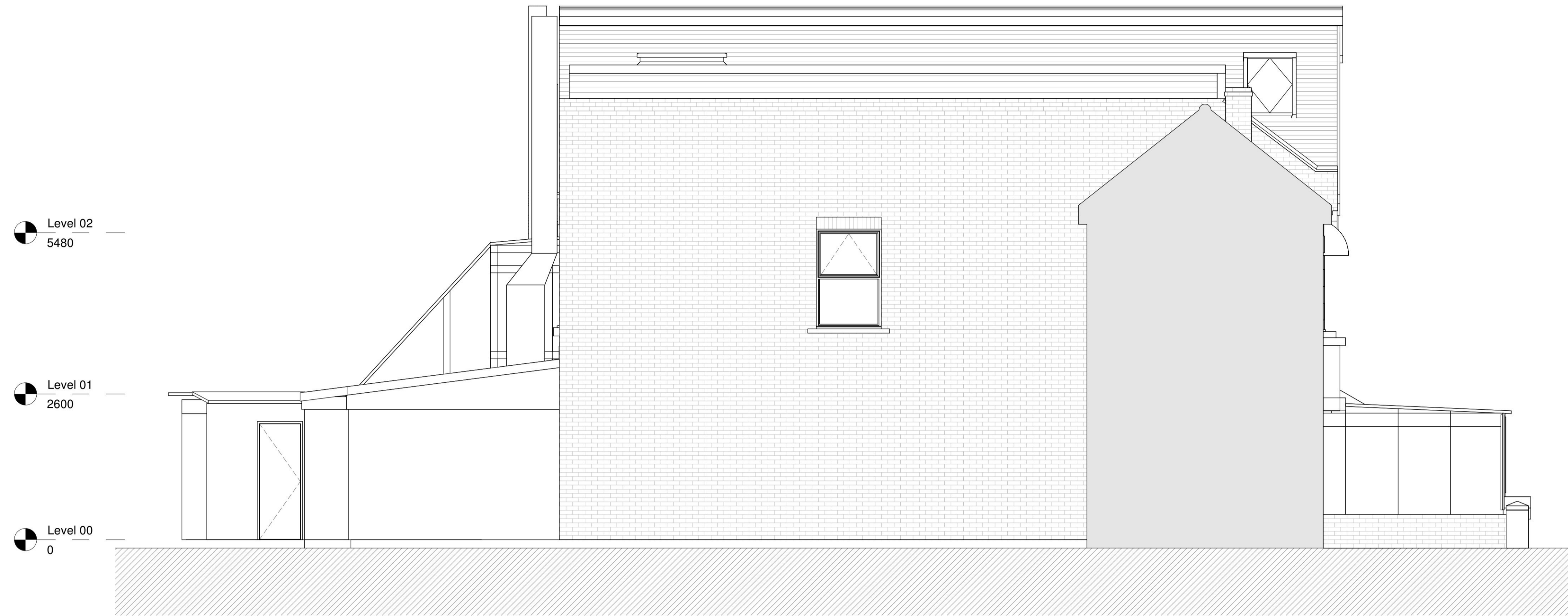
Side - East Elevation (Proposed)
