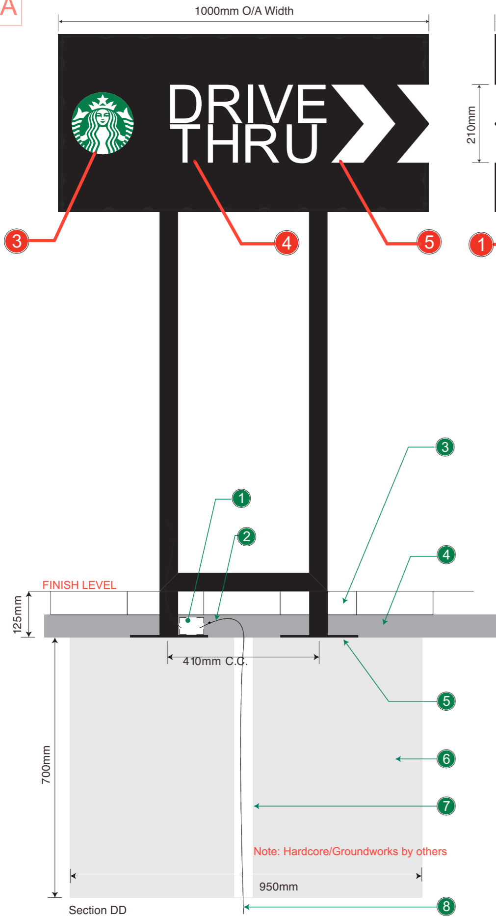
Base details
