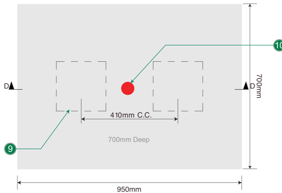
Base details
