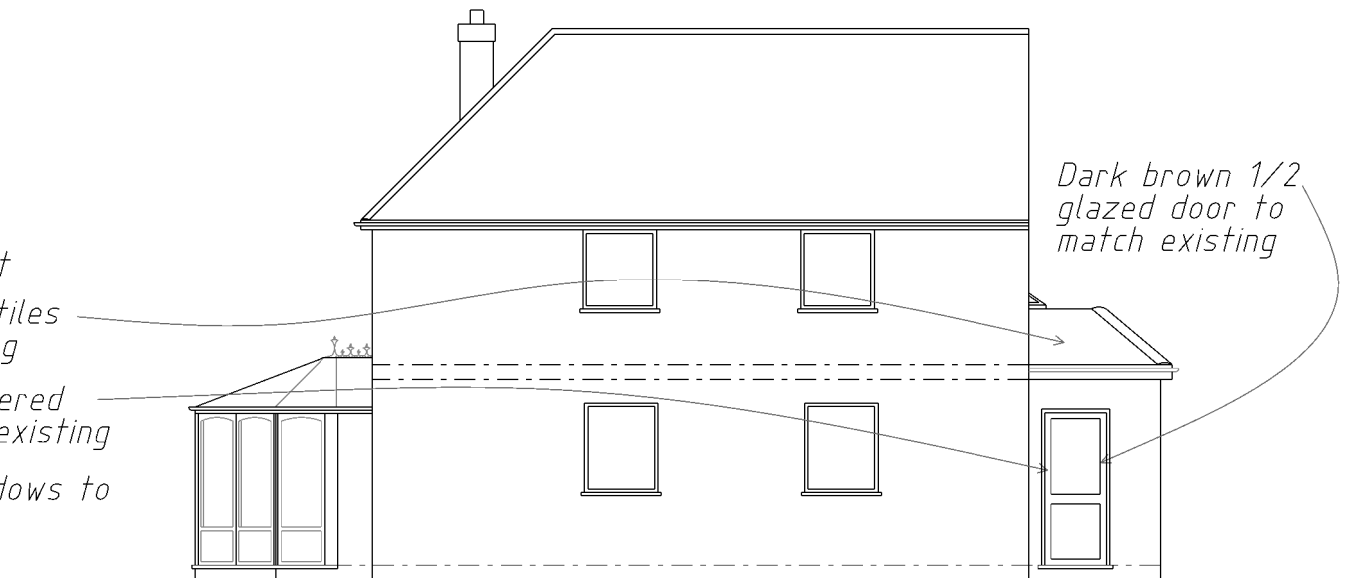
PROPOSED SIDE ( SW ) ELEVATION
