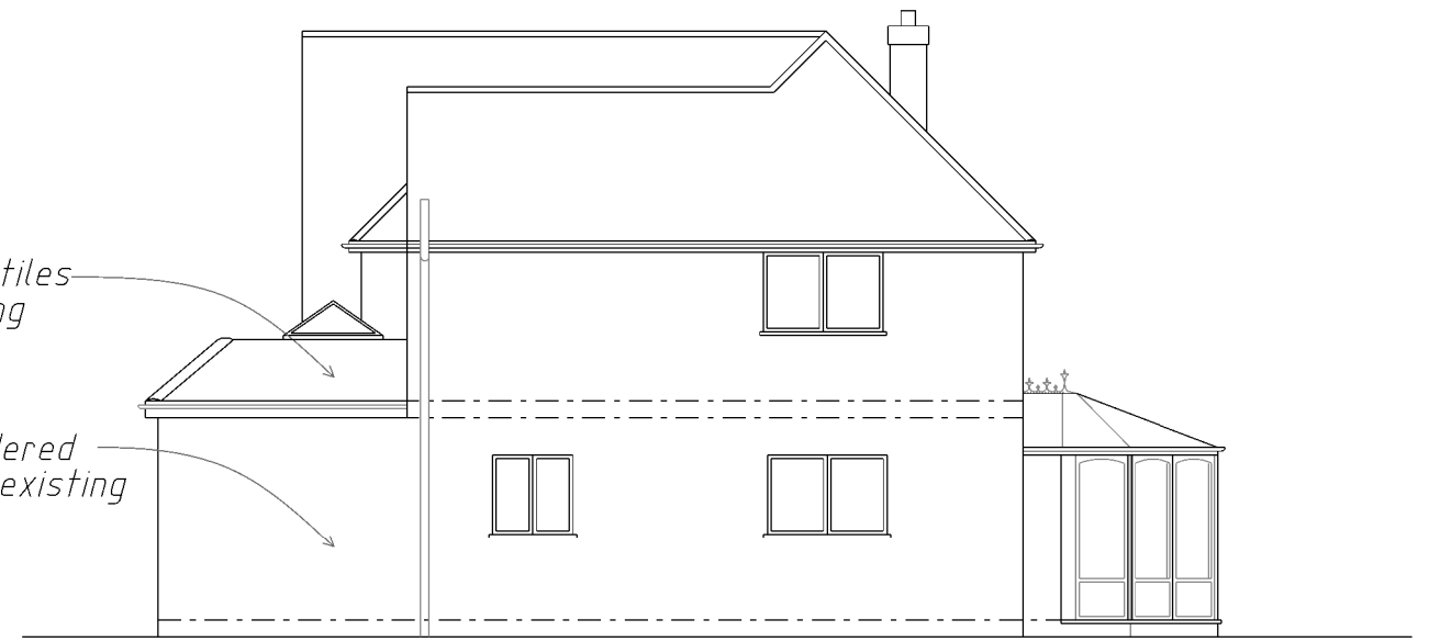
PROPOSED SIDE ( NE ) ELEVATION
