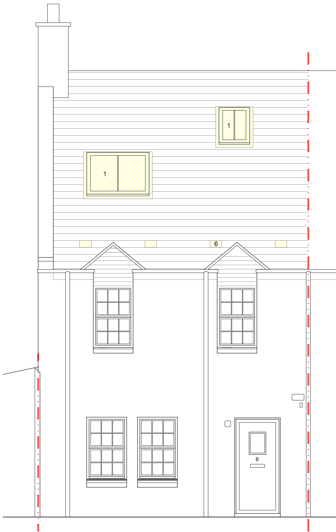
Proposed Front Elevation (W) 1:50
