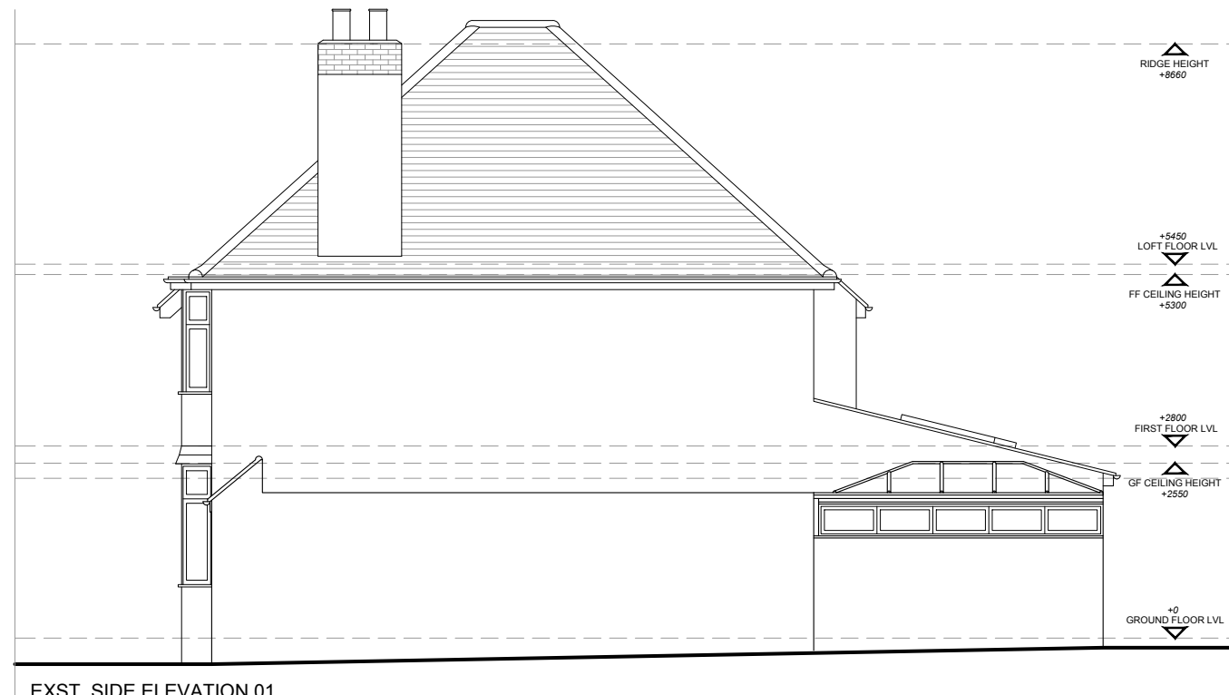
EXST. SIDE ELEVATION 01
