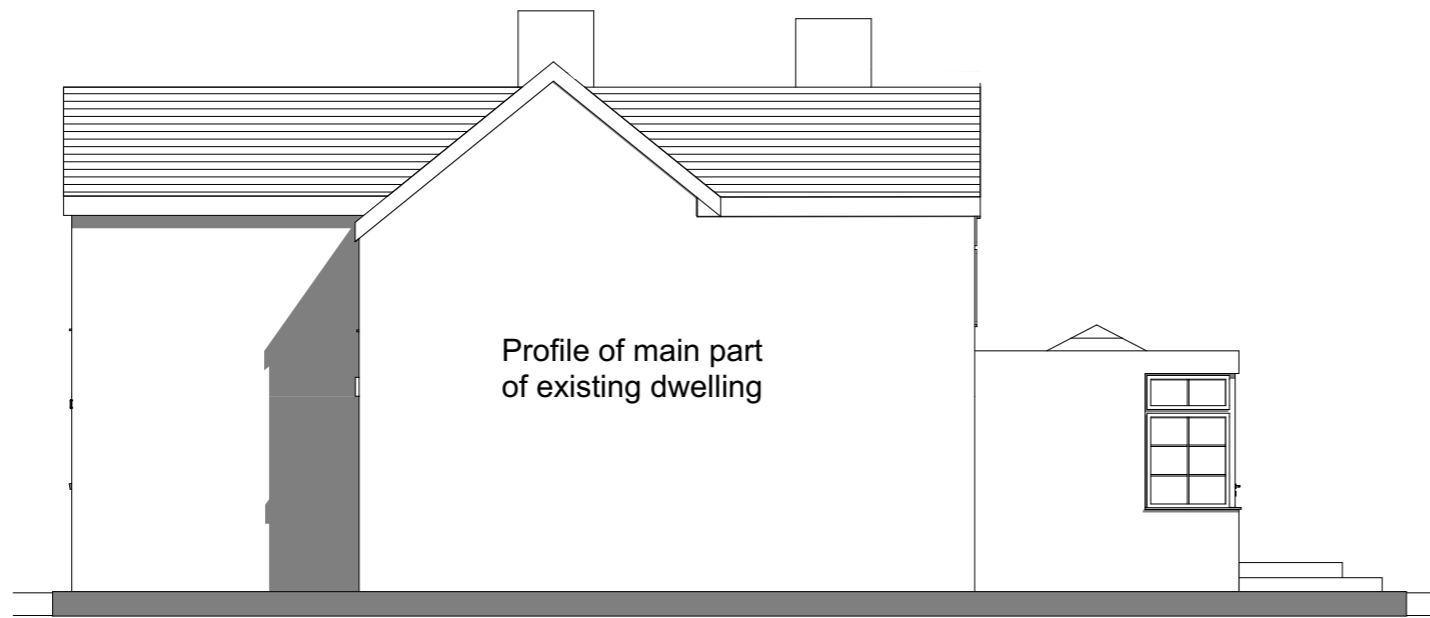
South Elevation
