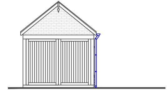
Proposed Front Elevation Scale 1:100
