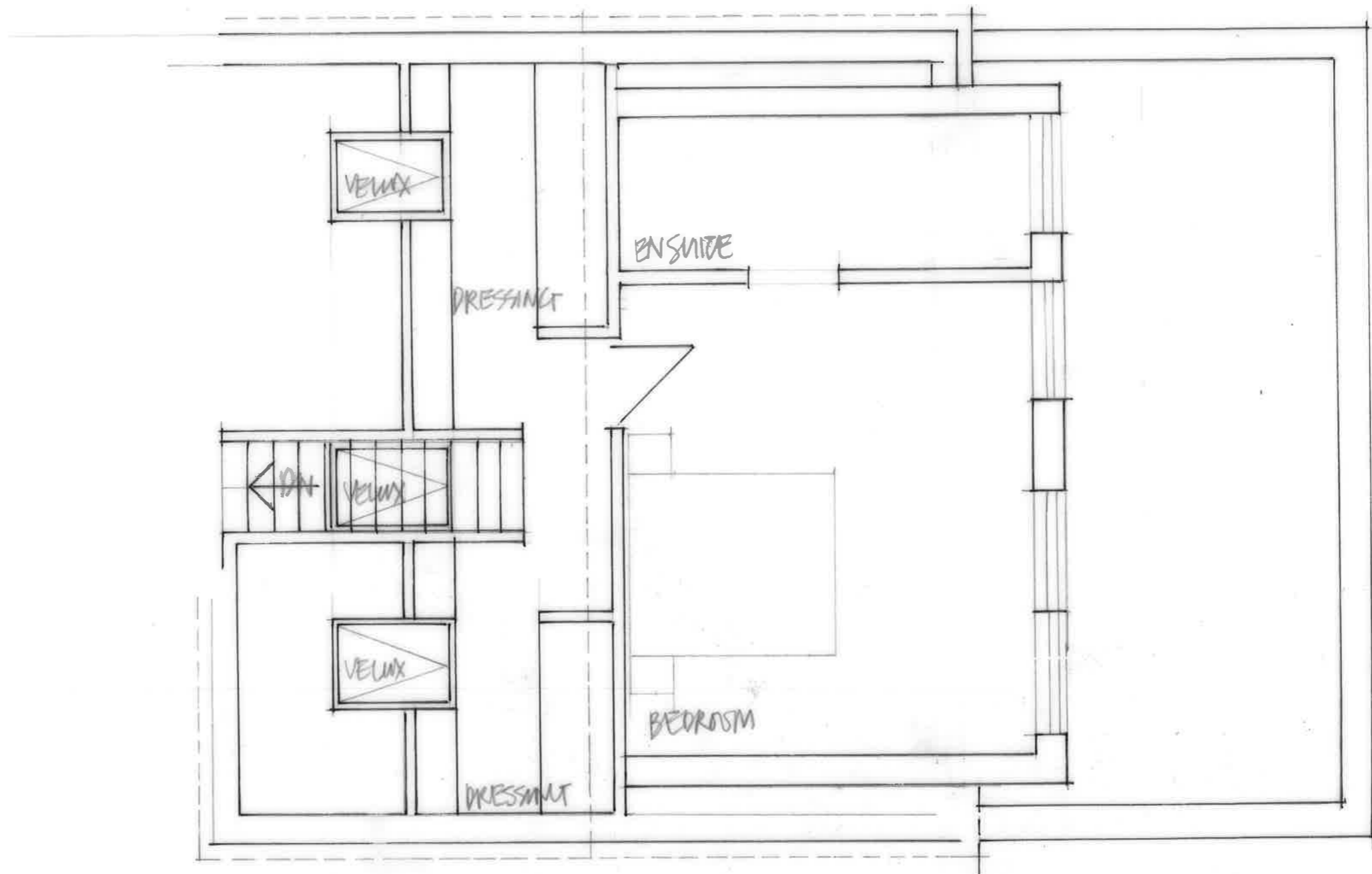
FIRST FLOOR PLAN AS PROPOSED 1:50
