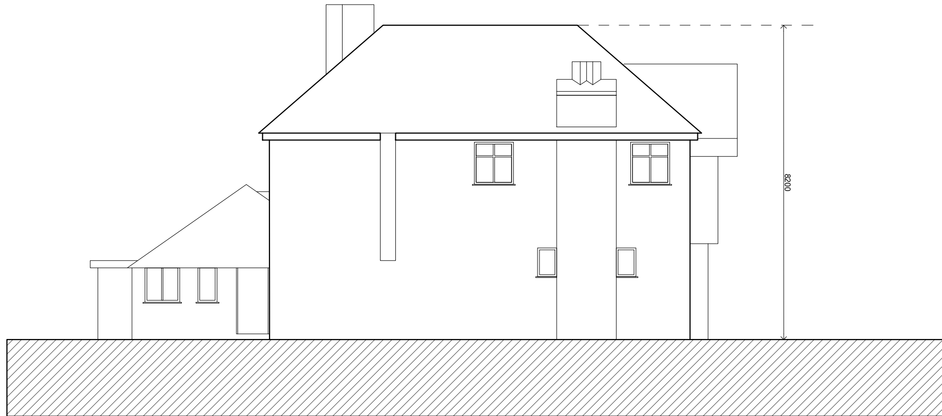
SIDE ELEVATION As seen from 77 The Ridgeway
