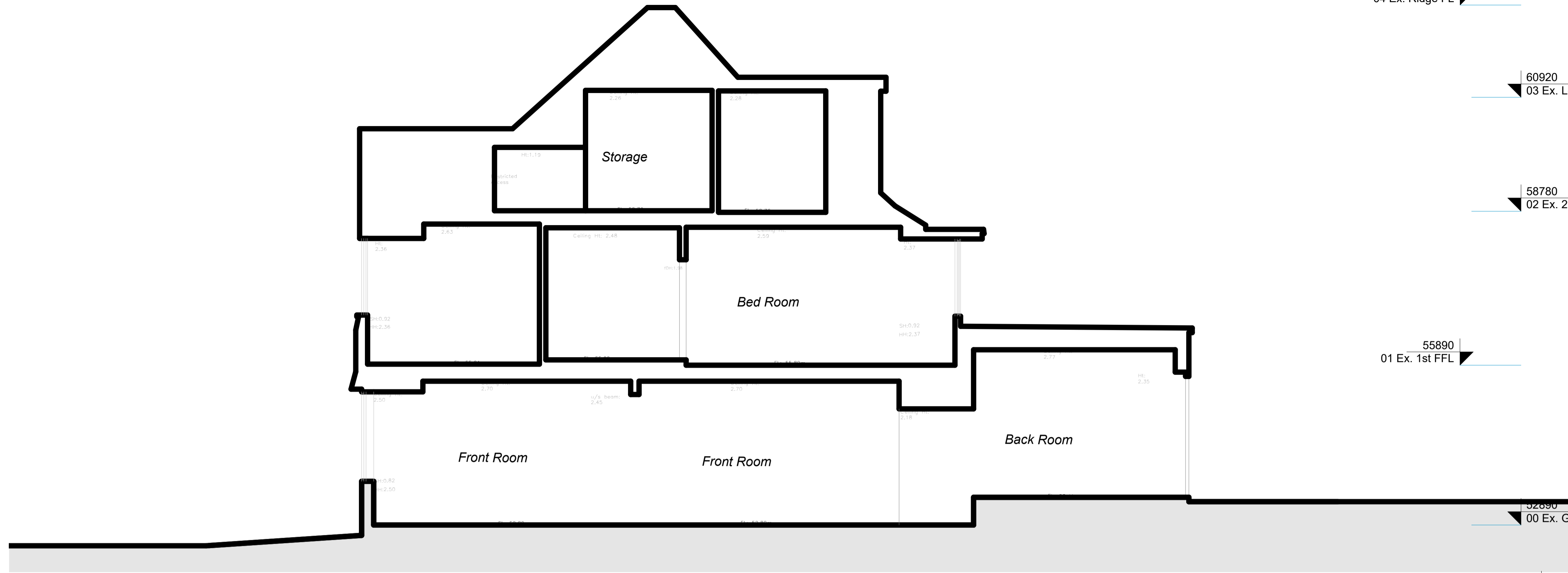
SC - Existing Section AA 1:50
