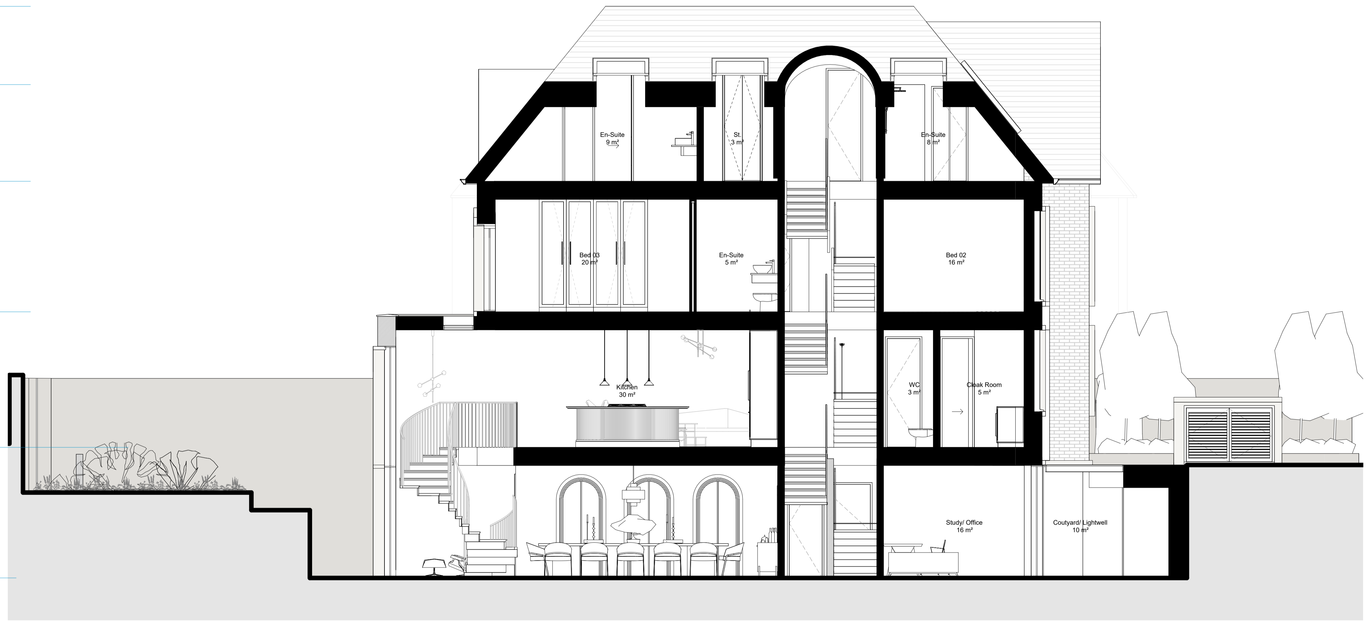
Proposed Section BB 1:50
