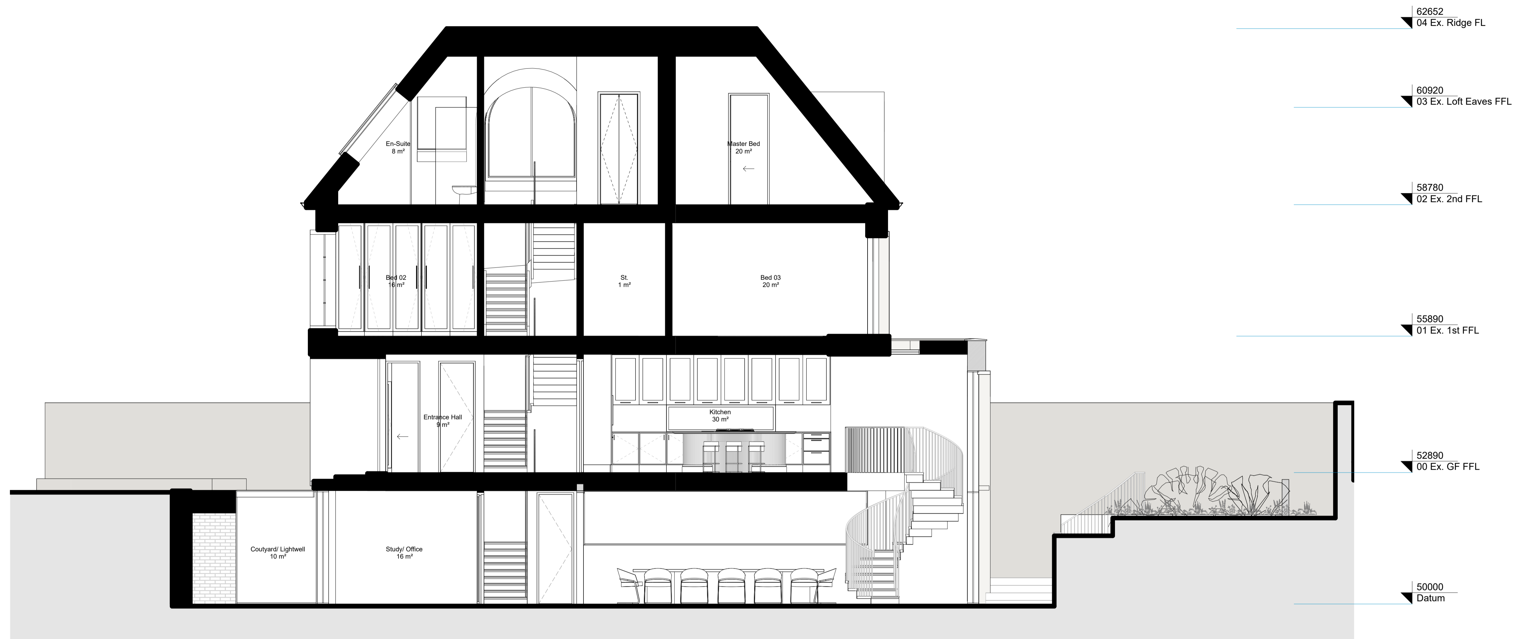
SC - Proposed Section AA 1:50
