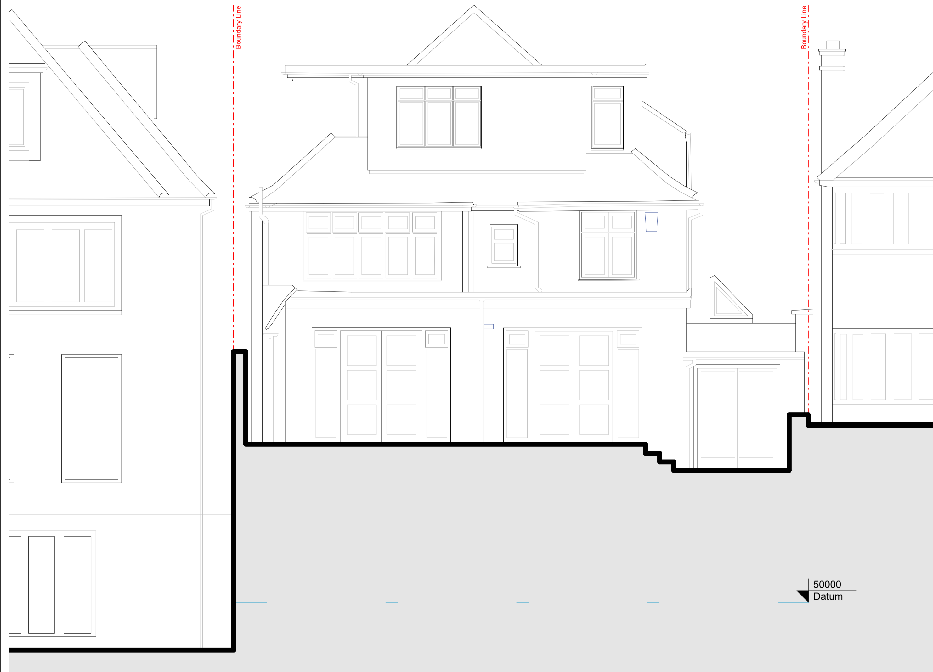
EL - Existing Rear Elevation
