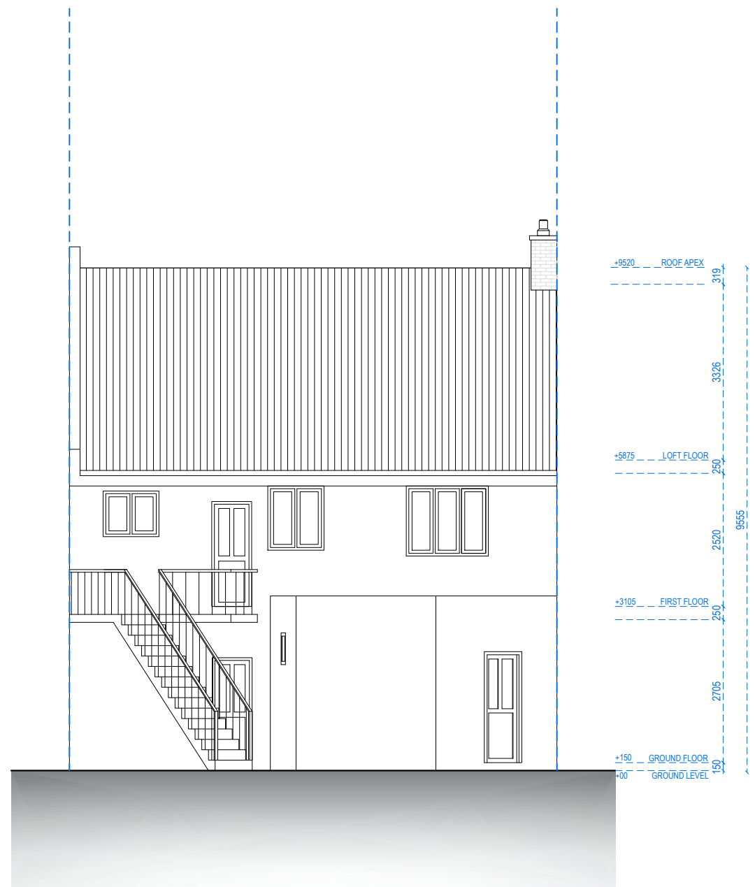
REAR ELEVATION
