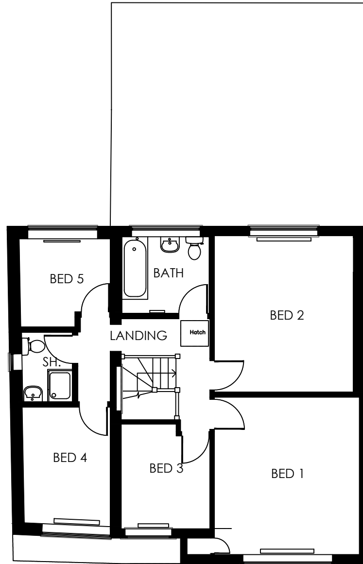
PROPOSED FIRST FLOOR SCALE - 1:100 @ A3
