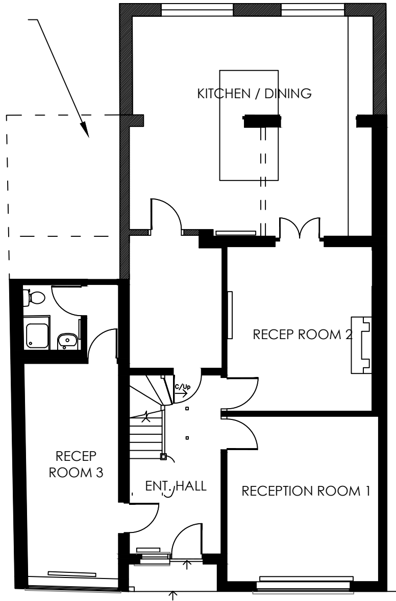
PROPOSED GROUND FLOOR SCALE - 1:100 @ A3
