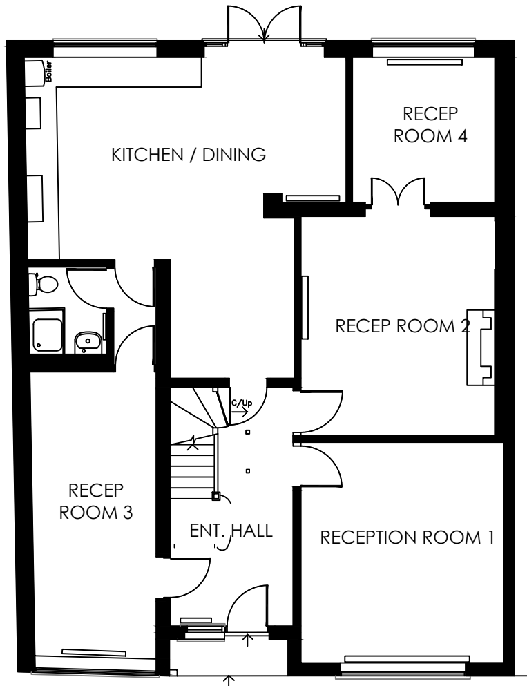
EXISTING GROUND FLOOR SCALE - 1:100 @ A3
