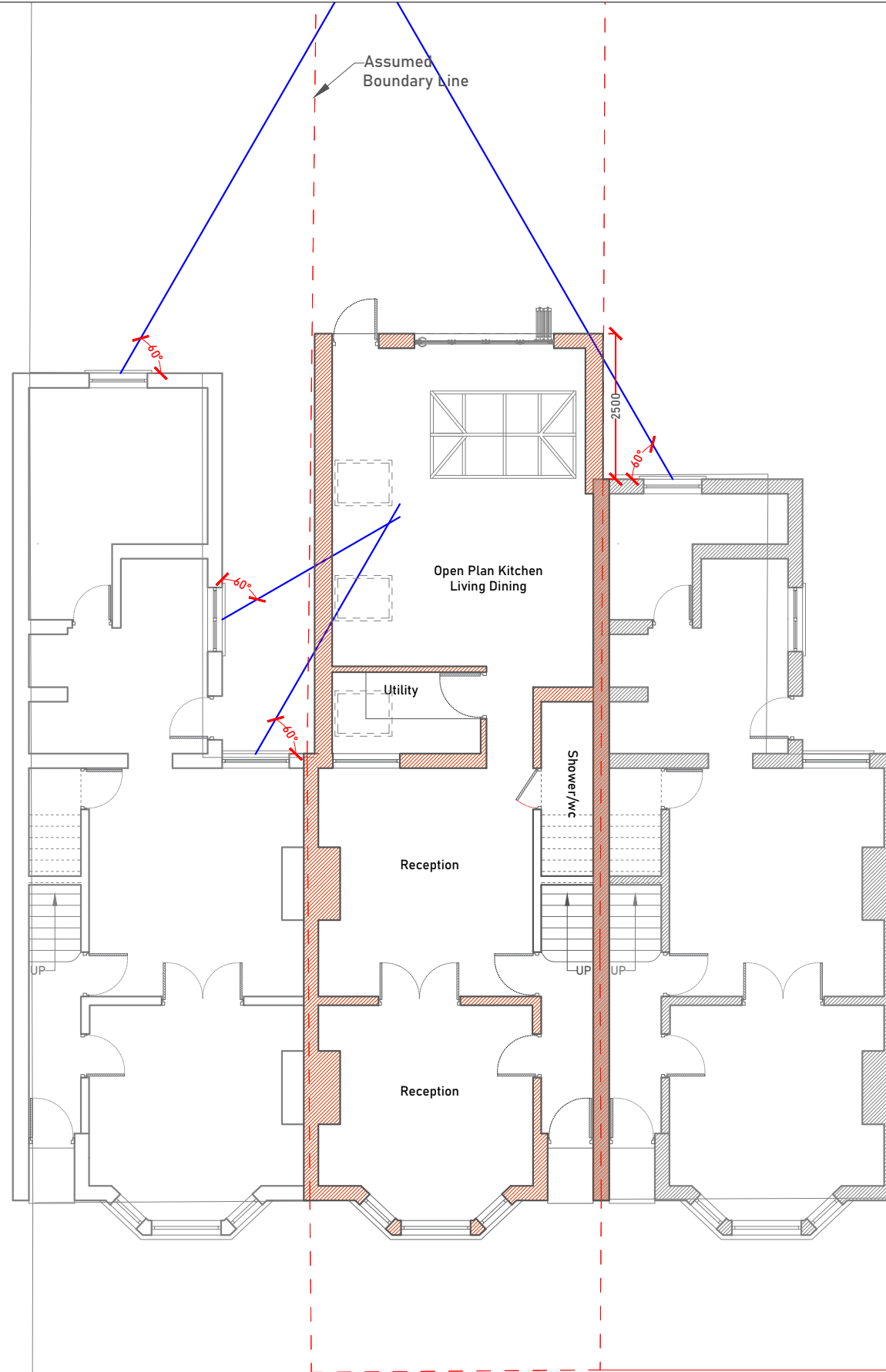
Proposed Ground Floor Plan 60 Degree angle
