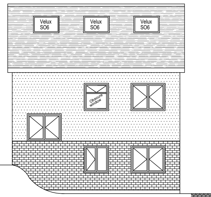
OPTION-4 FRONT ELEVATION NO CHANGE Scale:-1:100
