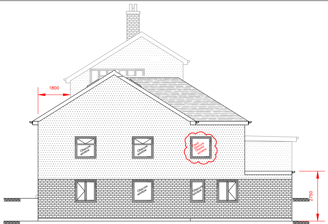
OPTION-4 SIDE WEST ELEVATION Scale:-1:100
