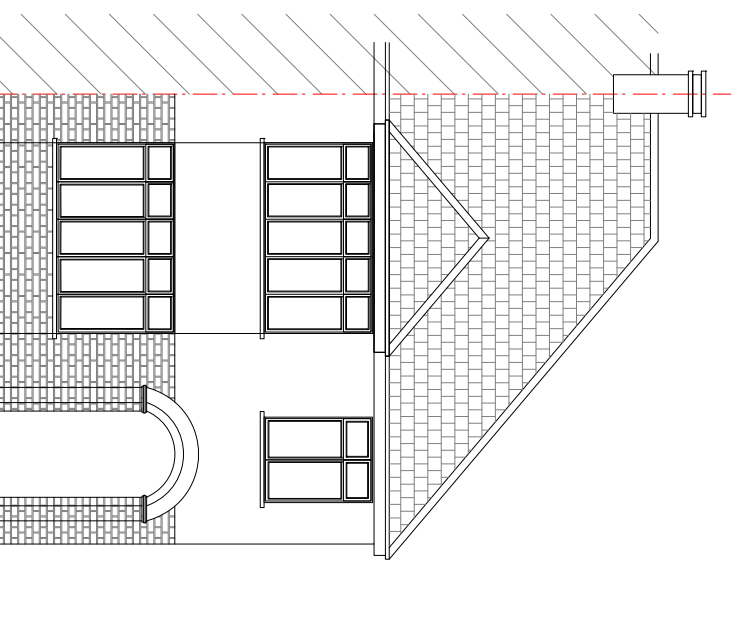
Front Elevation
