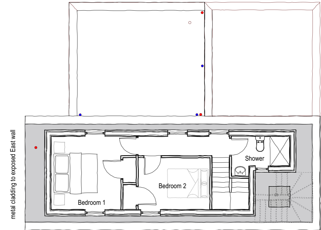
Proposed upward Extension
