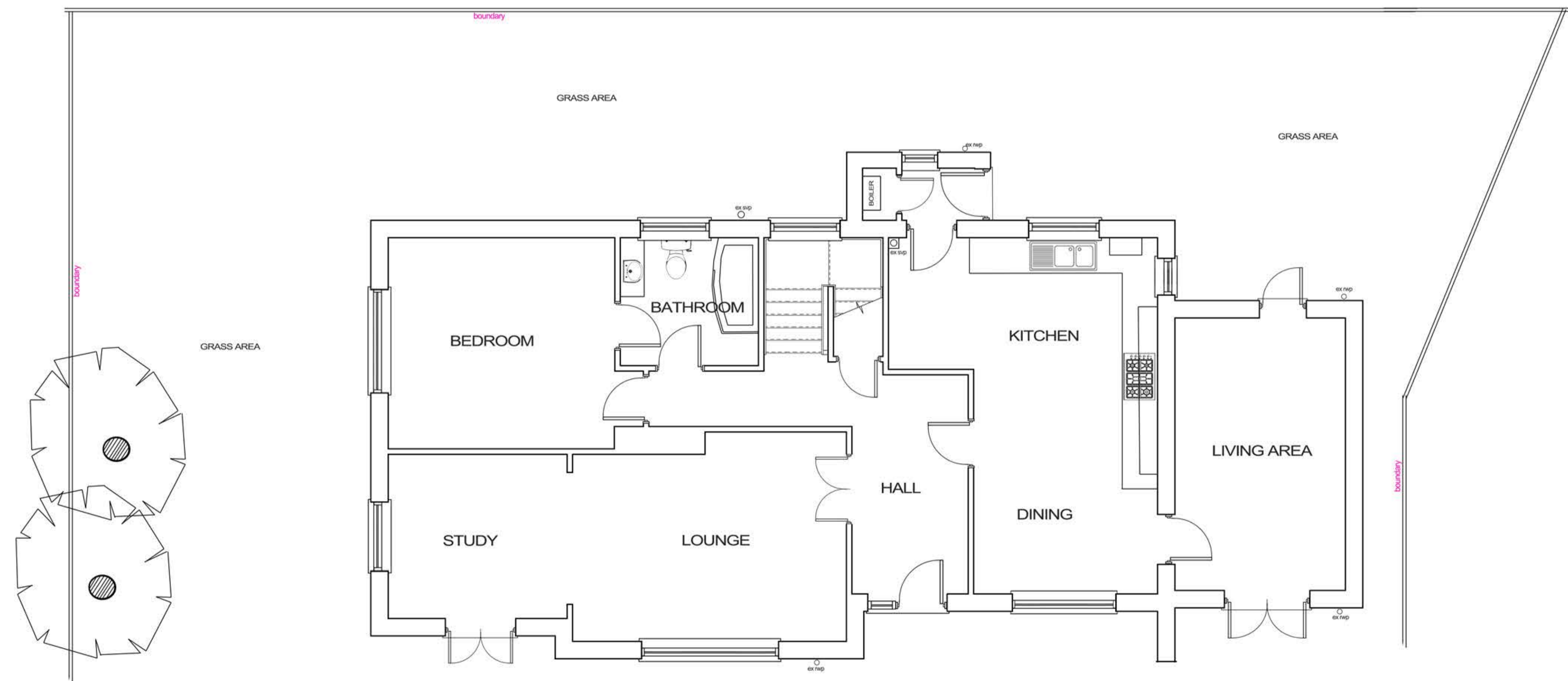
EXISTING GROUND FLOOR PLAN 1:50
