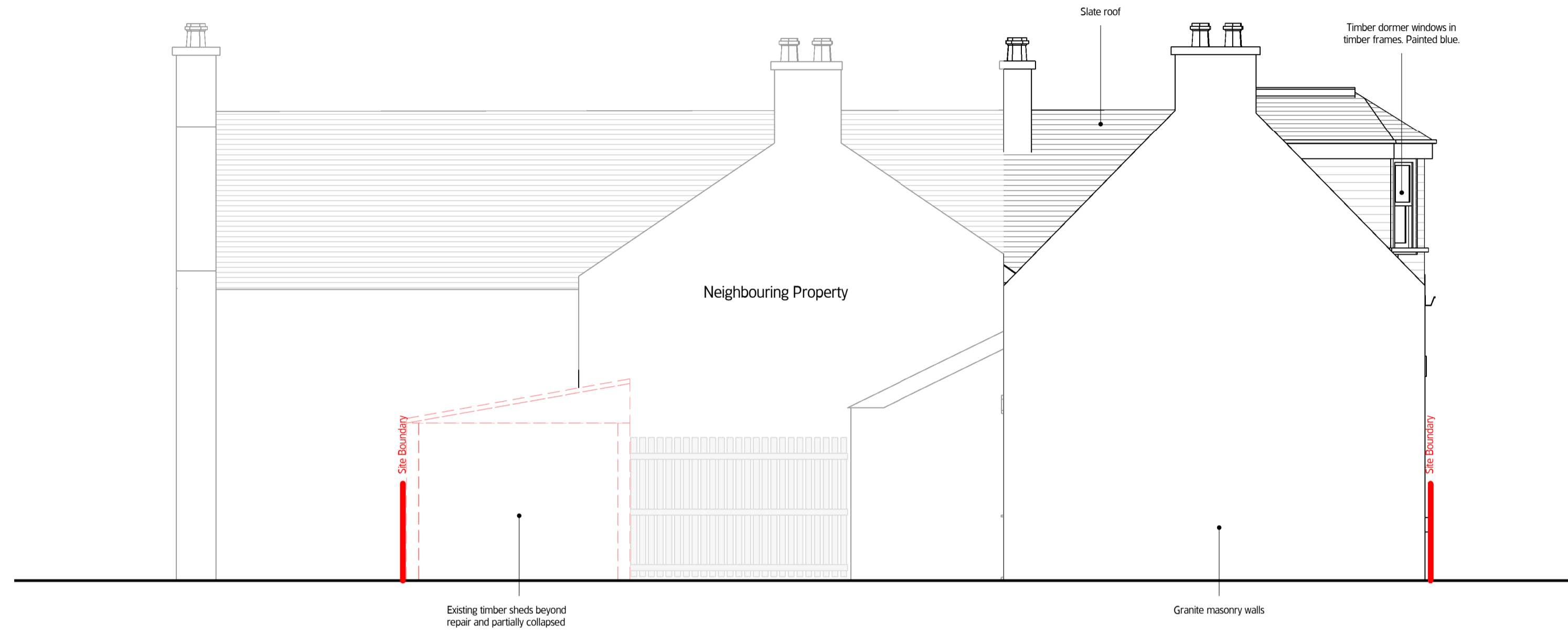
1 Elevation North - Existing 1 : 50
