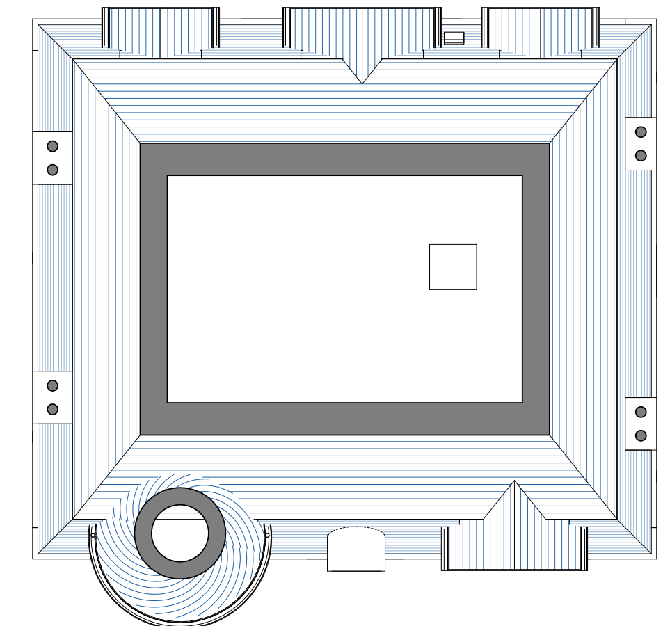
3 Proposed 02 Floor Level - Demo 1 : 100
