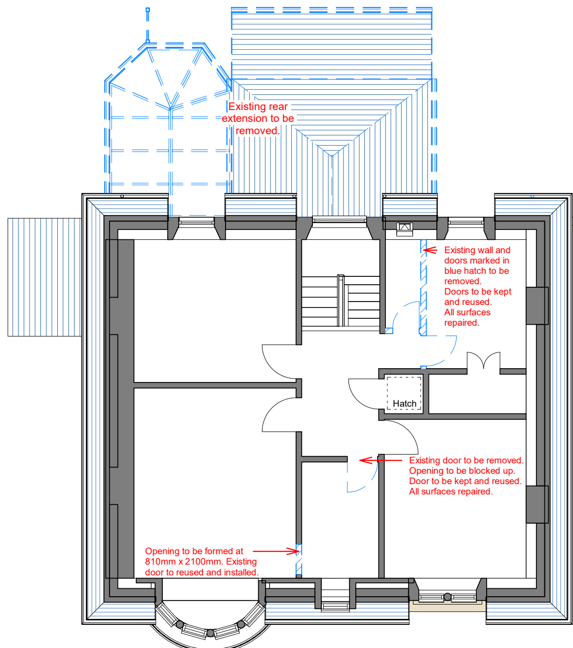
2 Proposed 01 Floor Level - Demo 1 : 100
