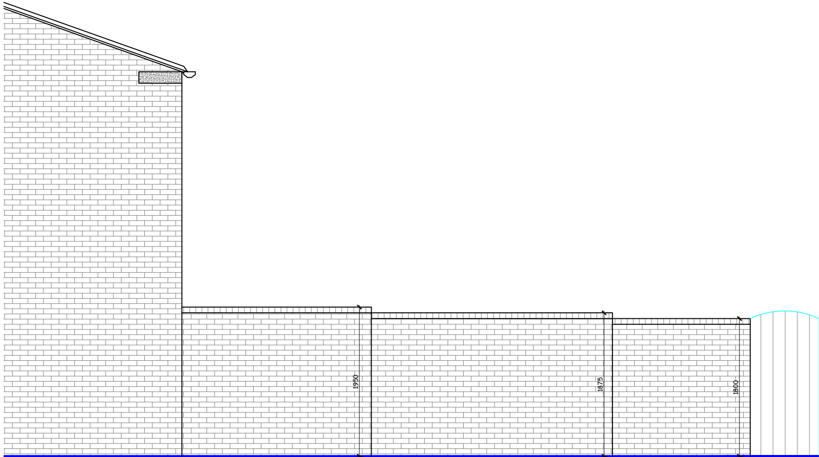
Existing Side Elevation - Boundary Treatment
