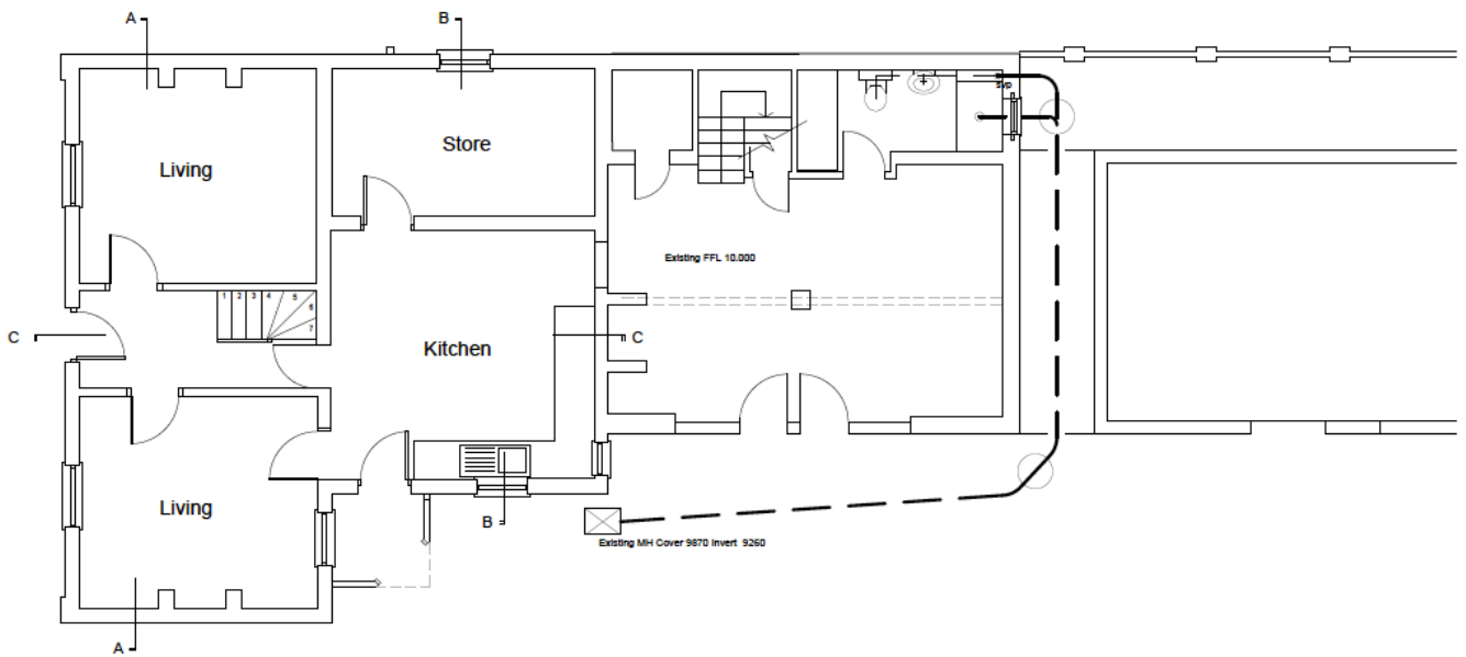
GRD FLOOR PLAN
